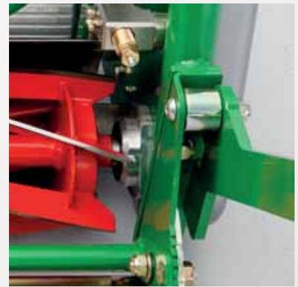
Easy adjustment of bottom blade to cylinder
