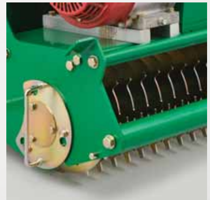
Simple changeover reel lock
